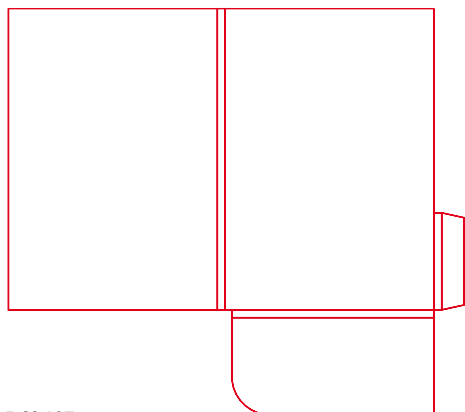
DAL137 Finished size (when closed): 215 x 309mm Flap: 100mm 8mm capacity
